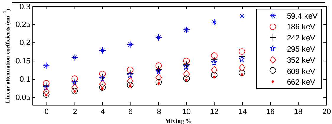
Fig 5. The relationship between the linear attenuation coefficient and mixing percentage.
