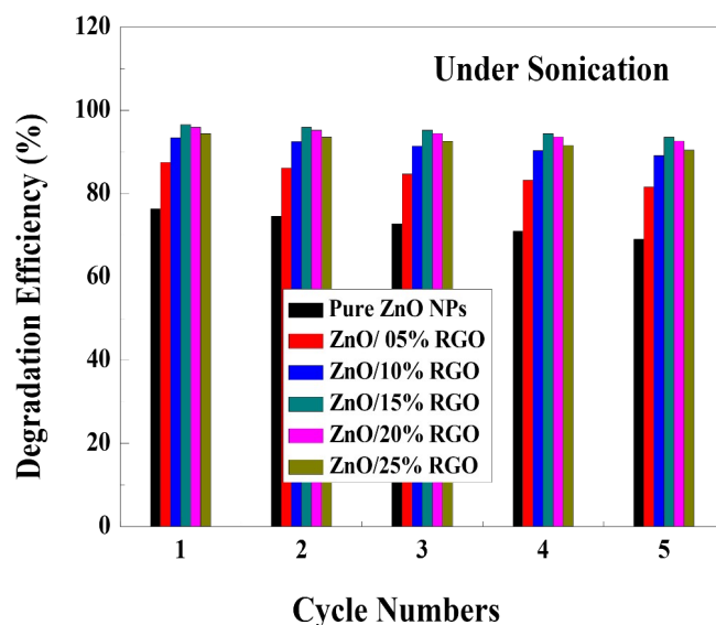
Figure 17 (b). Reusability performance and degradation efficiency of pristine ZnO NPs and ZnO/RGO NCs with different RGO loadings during MB degradation under sonication over five successive cycles.
