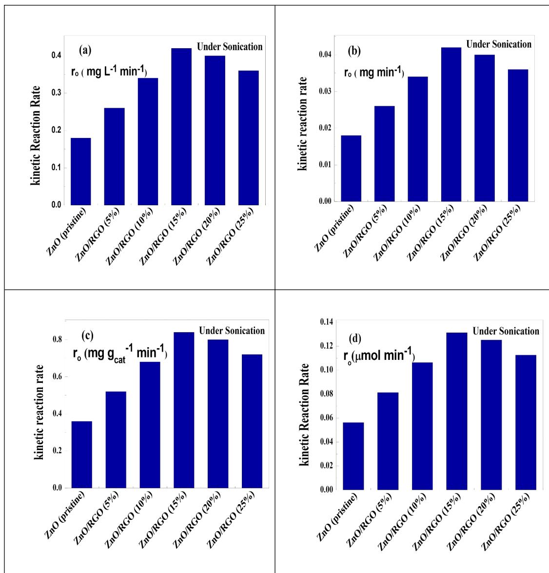
Figure 20. Initial reaction rates of pristine ZnO and ZnO/RGO NCs with varying RGO contents under sonication: (a) r_o(\text{mg L}^{-1} \text{min}^{-1}) is expressed as concentration over time. (b) r_o(\text{mg min}^{-1}) is expressed as mass over time. (c) r_o(\text{mg g}_{\text{cat}}^{-1} \text{min}^{-1}) is normalized to catalyst mass (d) r_o(\mu\text{mol min}^{-1}) is expressed in molar units under sonication.
