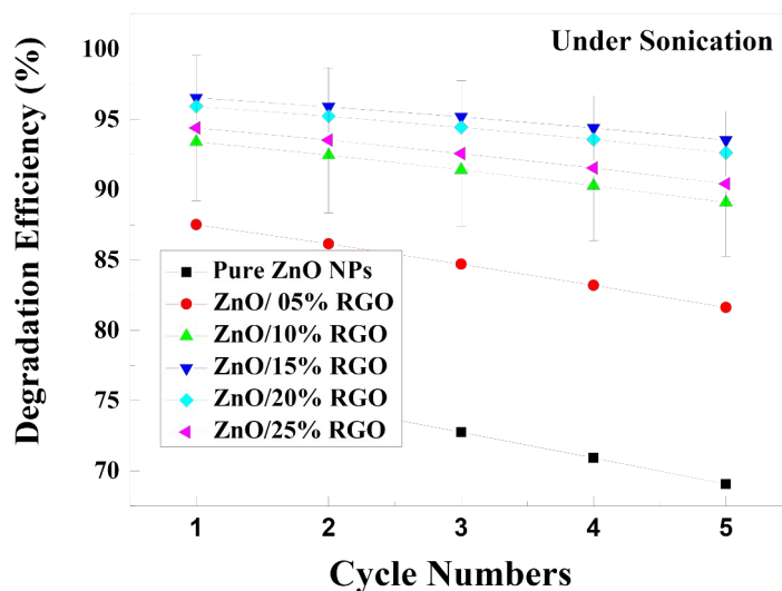
Figure 17 (a). Recyclability performance of pure ZnO NPs and ZnO/RGO NCs with varying RGO contents during sonocatalytic degradation of MB under ultrasonic irradiation over five consecutive cycles (each cycle conducted in triplicate, n = 3 ; data expressed as mean \pm standard deviation).
