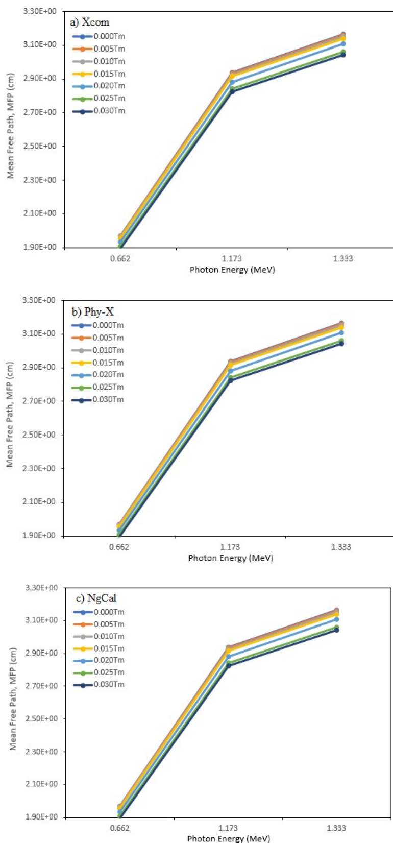
Figure 4. Graph mean free path Tm-doped borotellurite glass using a) Xcom, b) Phy-X, and c) NgCal
