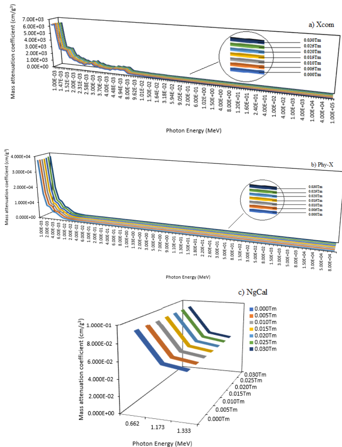
Figure 2. Graph mass attenuation coefficients of present glasses using a) Xcom, b) Phy-X, and c) NgCal
