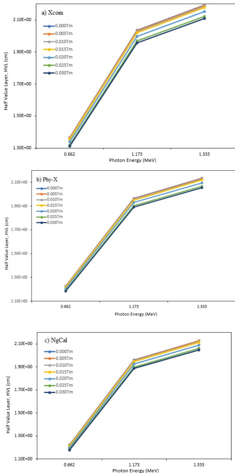
Figure 3. Graph half value layer Tm-doped borotellurite glass using a) Xcom, b) Phy-X, and c) NgCal
