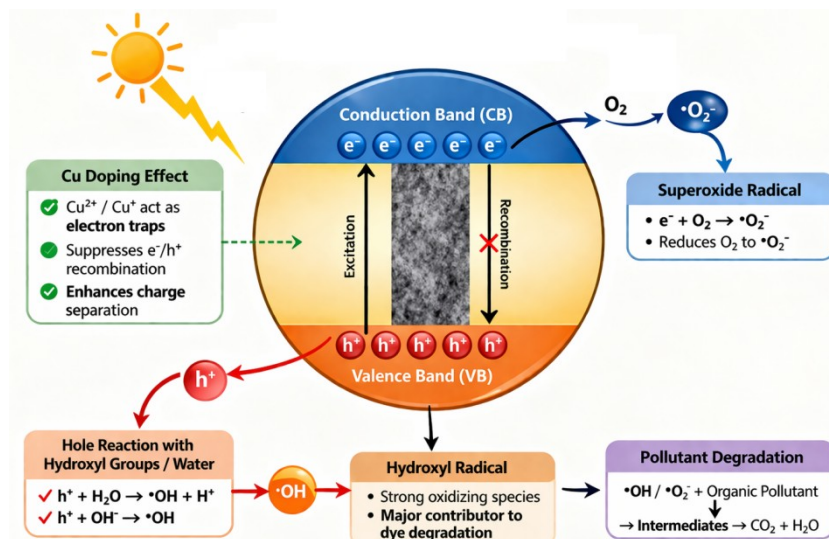
Figure 7. Proposed photocatalytic mechanism of pollutant (MB dye) using Cu-d-ZnO under UV light irradiation.
