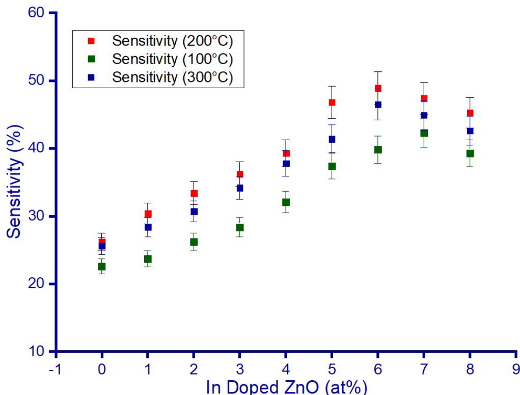
Figure 5. Sensitivity of In Doped ZnO thin films (0-8 at%) at different temperatures.
