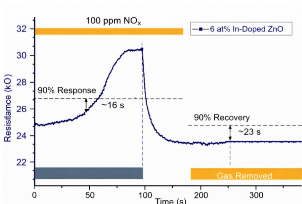
Figure 6. Response/recovery of 6 at% In Doped ZnO towards \text{NO}_x gas measured at the operating temperature 200^\circ\text{C} .
