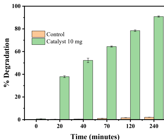
Figure 6. Photocatalytic degradation of dye using ZnO NPs under light irradiation.
