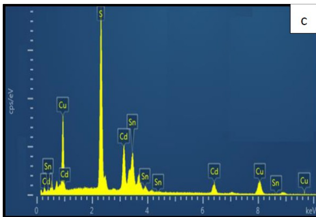
Figure 3. EDXA spectra of \text{Cu}_2\text{Cd}_x\text{Zn}_{1-x}\text{SnS}_4 alloys for (a) x=0.0 , (b) x=0.5 , and (c) x=1.0
