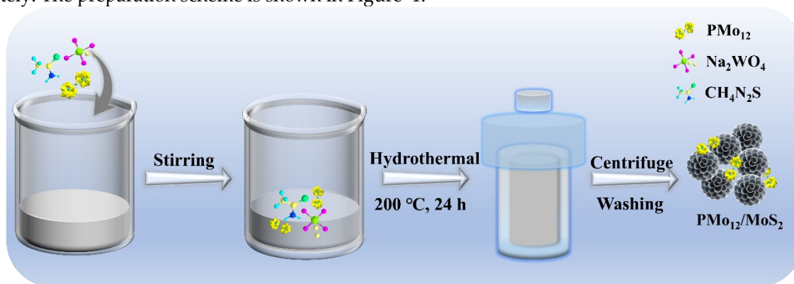
Figure 1. Schematic illustration of the synthesis process of \text{PMo}_{12}/\text{MoS}_2 composites.
